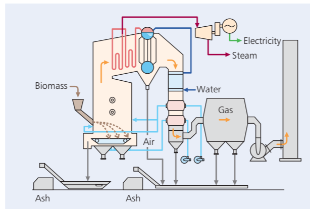
Bagasse-fired boiler installation example
