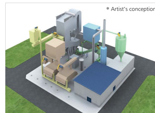
Installation example (Tama River Water Recycling Center [currently under construction], Tokyo)
